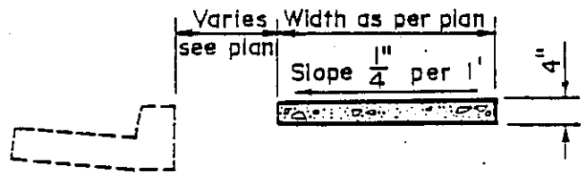
TYPE "F" CURB
