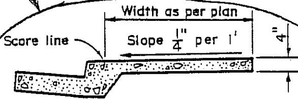
TYPE "E" CURB
